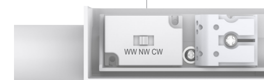
CCT Selection DIP Switch
